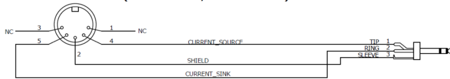
TRS to MIDI adapter Female DIN5 (Connector, front view)
